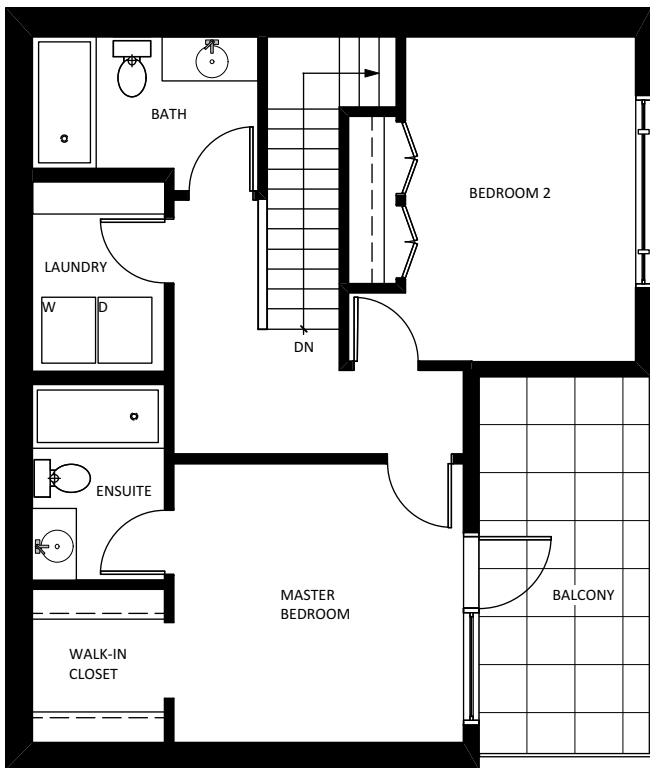
UPPER FLOOR
